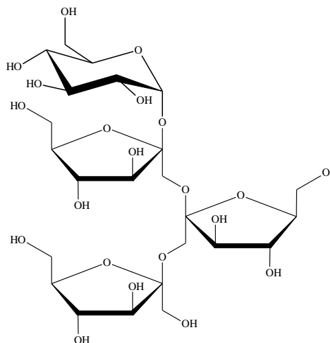
O- \beta -D-fructofuranosyl-(2-1)- \beta -D-fructofuranosyl-(2-1)- \beta -D-fructofuranosyl- \alpha -D-glucopyranoside
