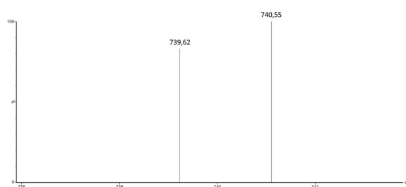
MS spectrum of LIB'UP® U-[13C34]-Fumonisin B2
