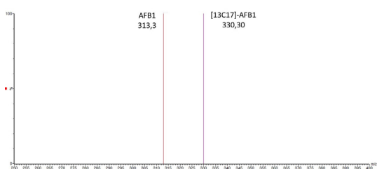
MS spectrum of Aflatoxin B1 and standard LIB'UP® U-[13C17]-Aflatoxin B1
