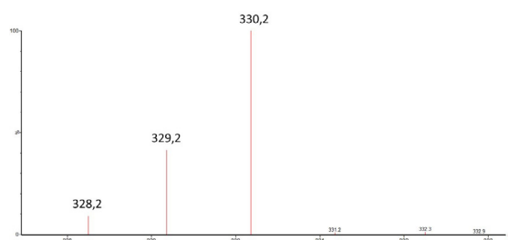
MS spectrum of LIB'UP® U-[13C17]-Aflatoxin B1
